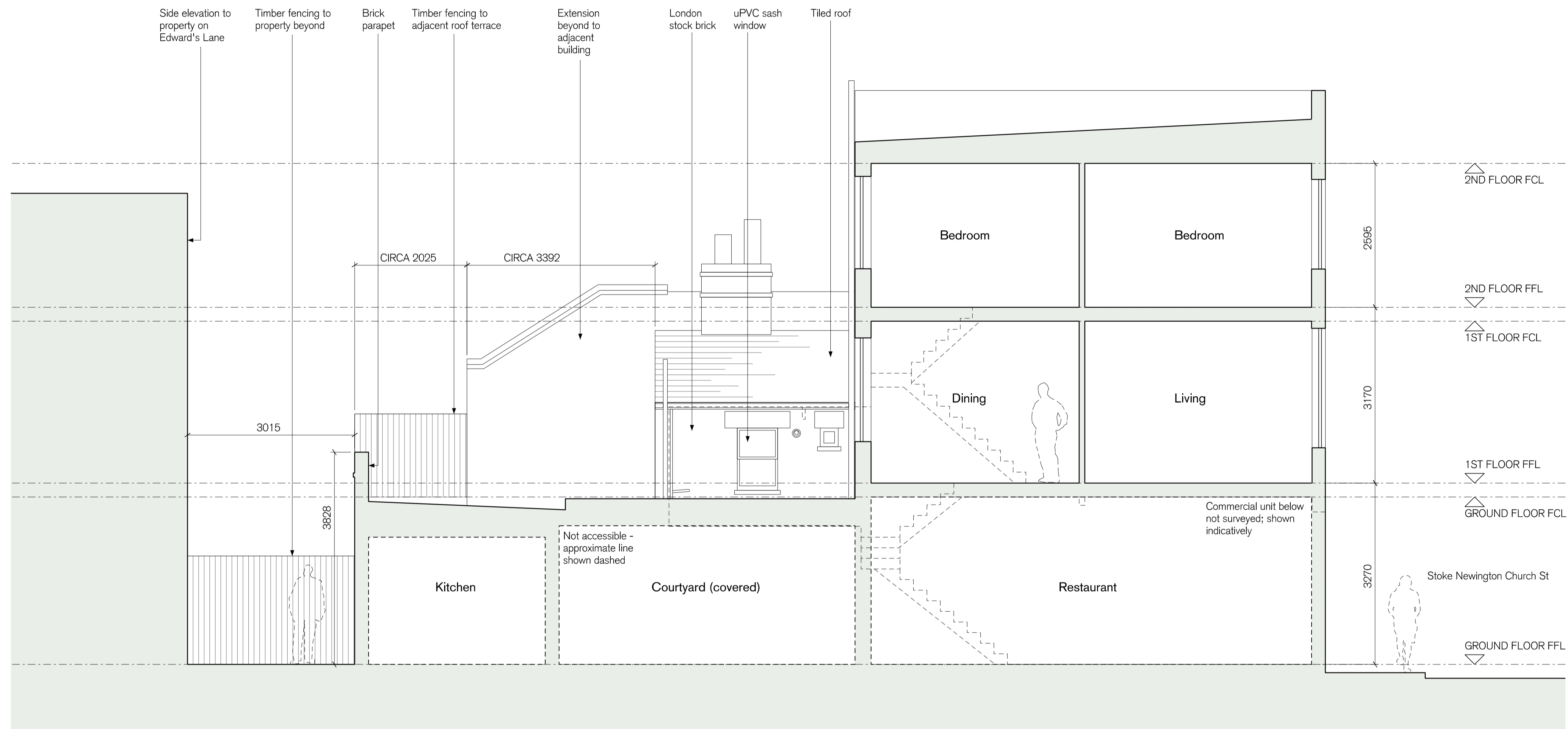
Long section A
