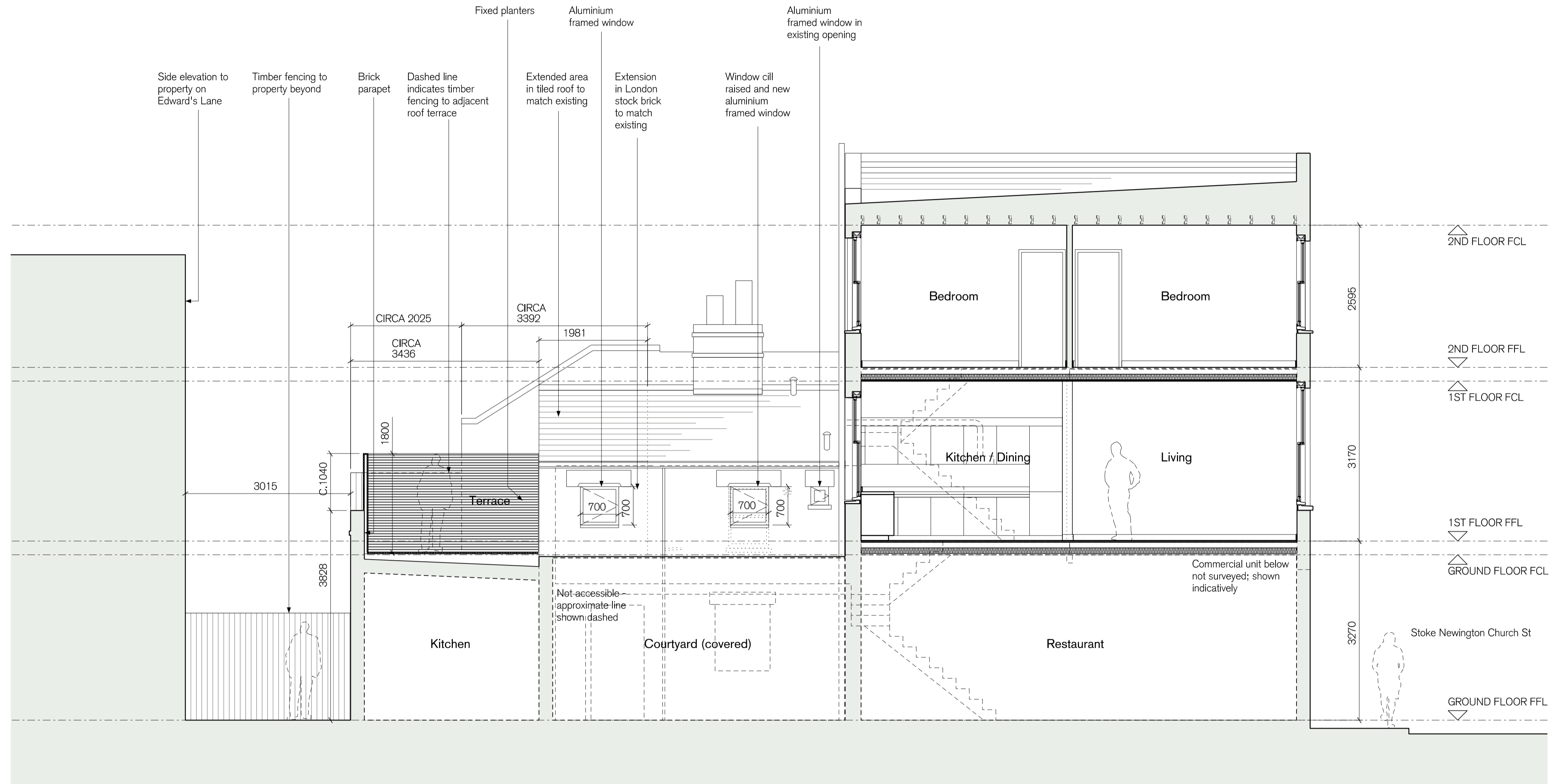
Long section A
